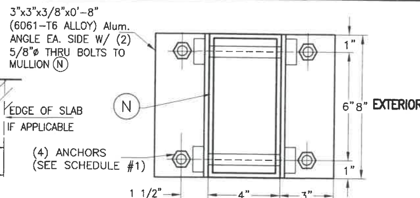
ALTERNATIVE SECTION X1-X1 W/ (N) *
