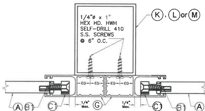
SECTION R-R :MULLION MOUNT (FACE MOUNT) SCALE: 3/8" = 1"
