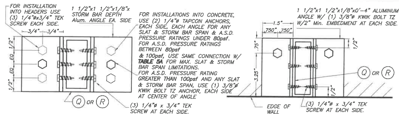
SECTION S2 - S2
