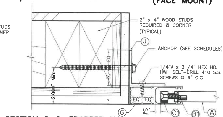
SECTION O-O: TRAPPED MOUNT SCALE: 3/8" = 1"
