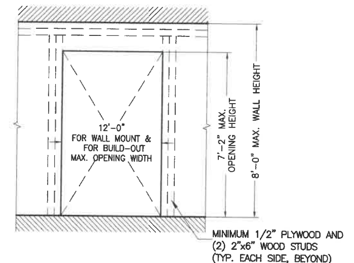
DETAIL 1 (ELEVATION)
