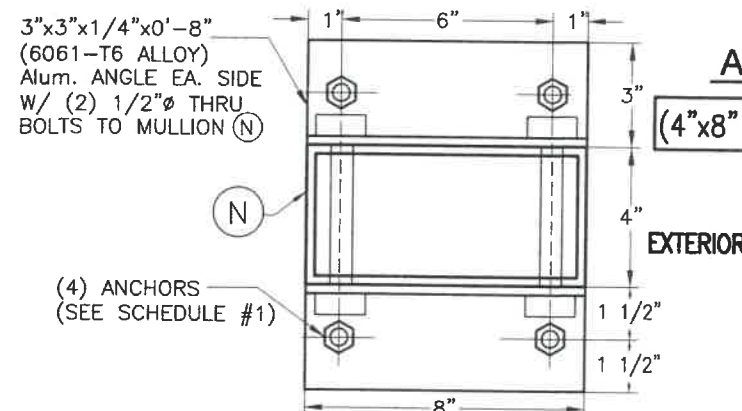
ALTERNATIVE SECTION X1-X1 W/ (N) *
