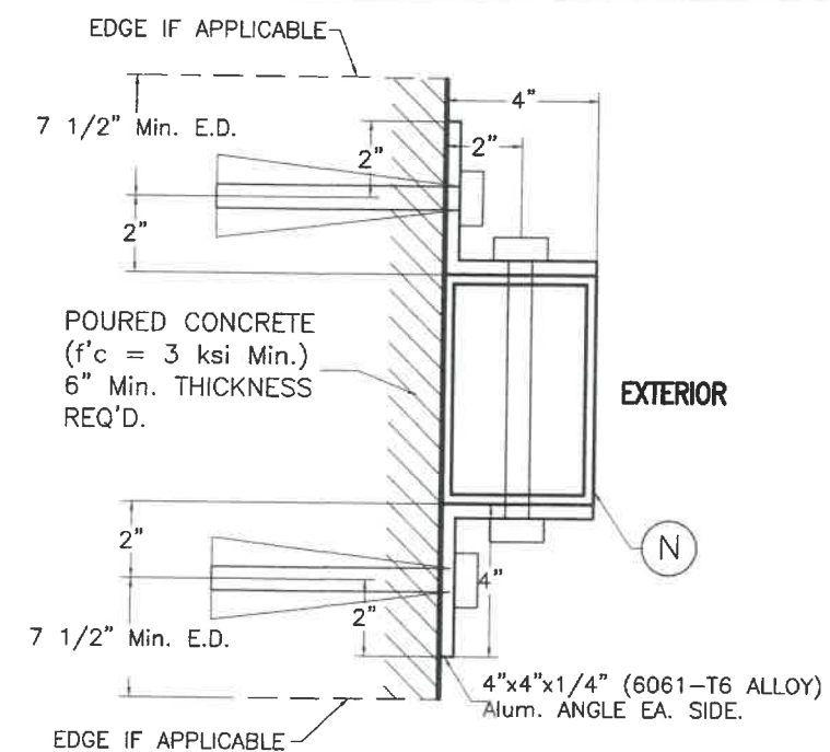
ALTERNATIVE SECTION X2-X2 W/ (N) * (END & INTERIOR MULLIONS) (W/ ORIENTATION # 1) (8"x4")
