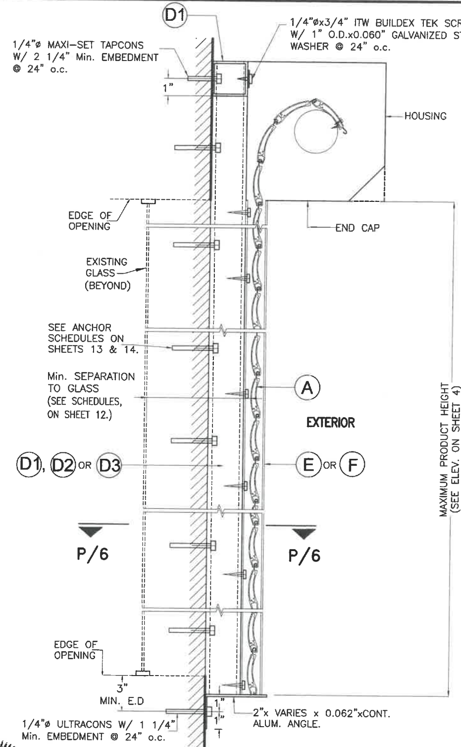
BUILD-OUT MOUNTING
