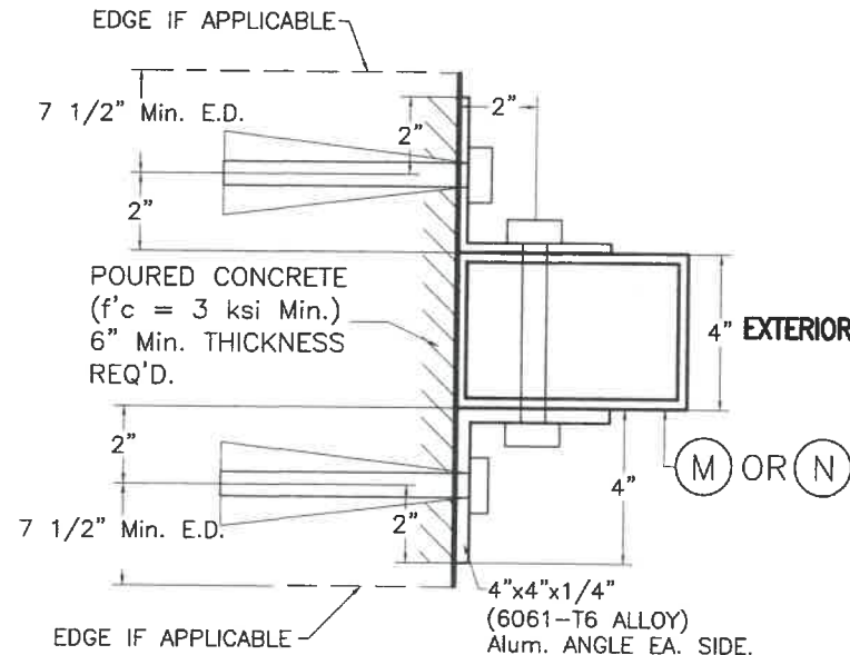
ALTERNATIVE SECTION X2-X2 W/ (M) OR (N) * (INTERIOR MULLION) (W/ ORIENTATION # 2) (4"x6" or 4"x8")
