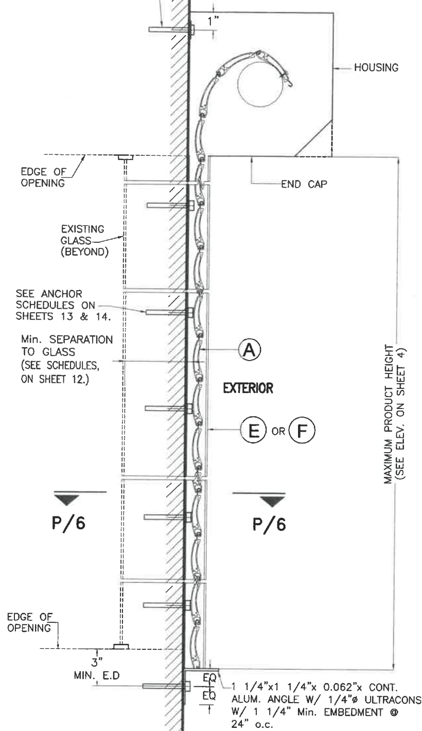
WALL MOUNTING
