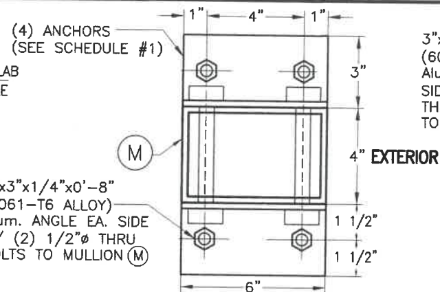
ALTERNATIVE SECTION X1-X1 W/ (M) *
