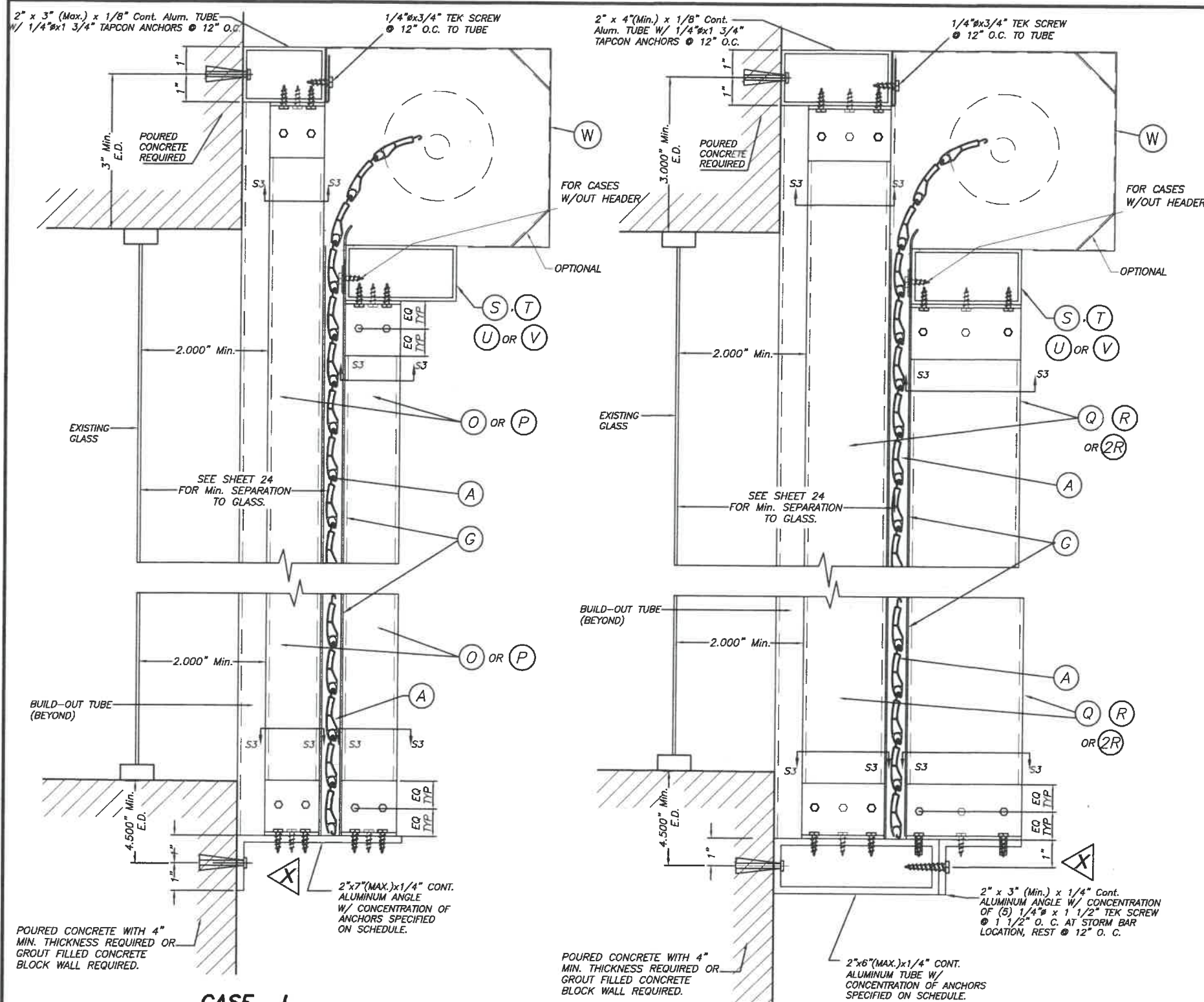
CASE I FIXED STORM BAR CONNECTION AT BUILD-OUT INSTALLATIONS W/SHEET METAL SCREWS OR MACHINE SCREWS SCALE : 1/4" = 1"
