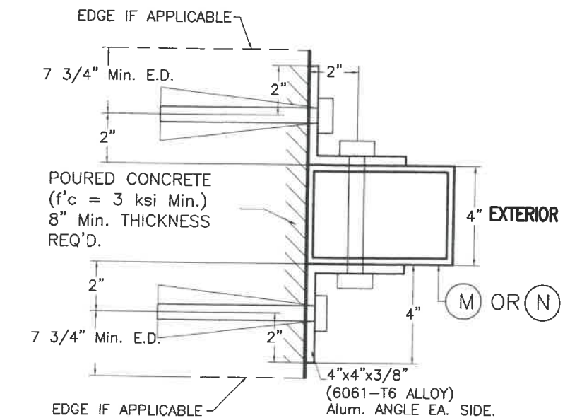
ALTERNATIVE SECTION X2-X2 W/ (M) OR (N)* (END & INTERIOR MULLION) (W/ ORIENTATION # 2) (4"x6" or 4"x8")
