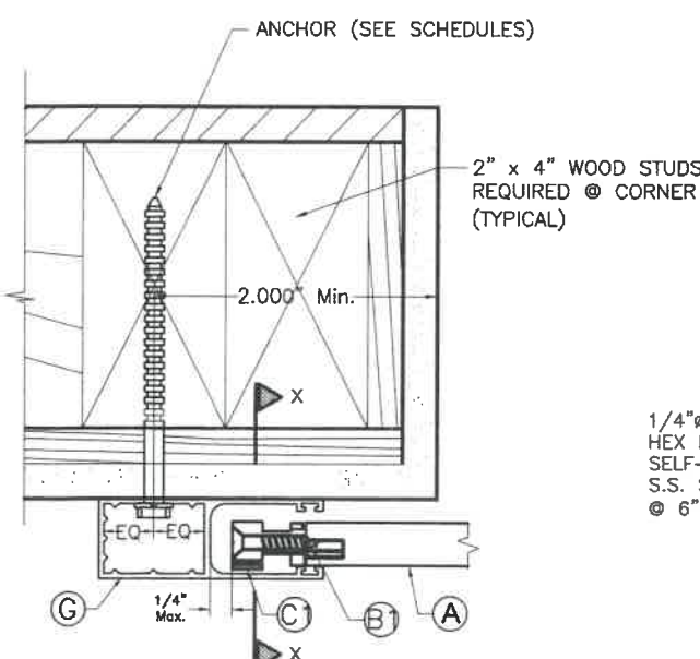
SECTION O-O: WALL MOUNT SCALE: 3/8" = 1"
